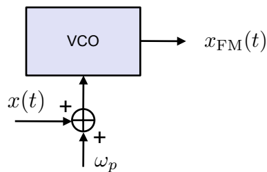
Modulateur FM: Voltage Controlled Oscillator
